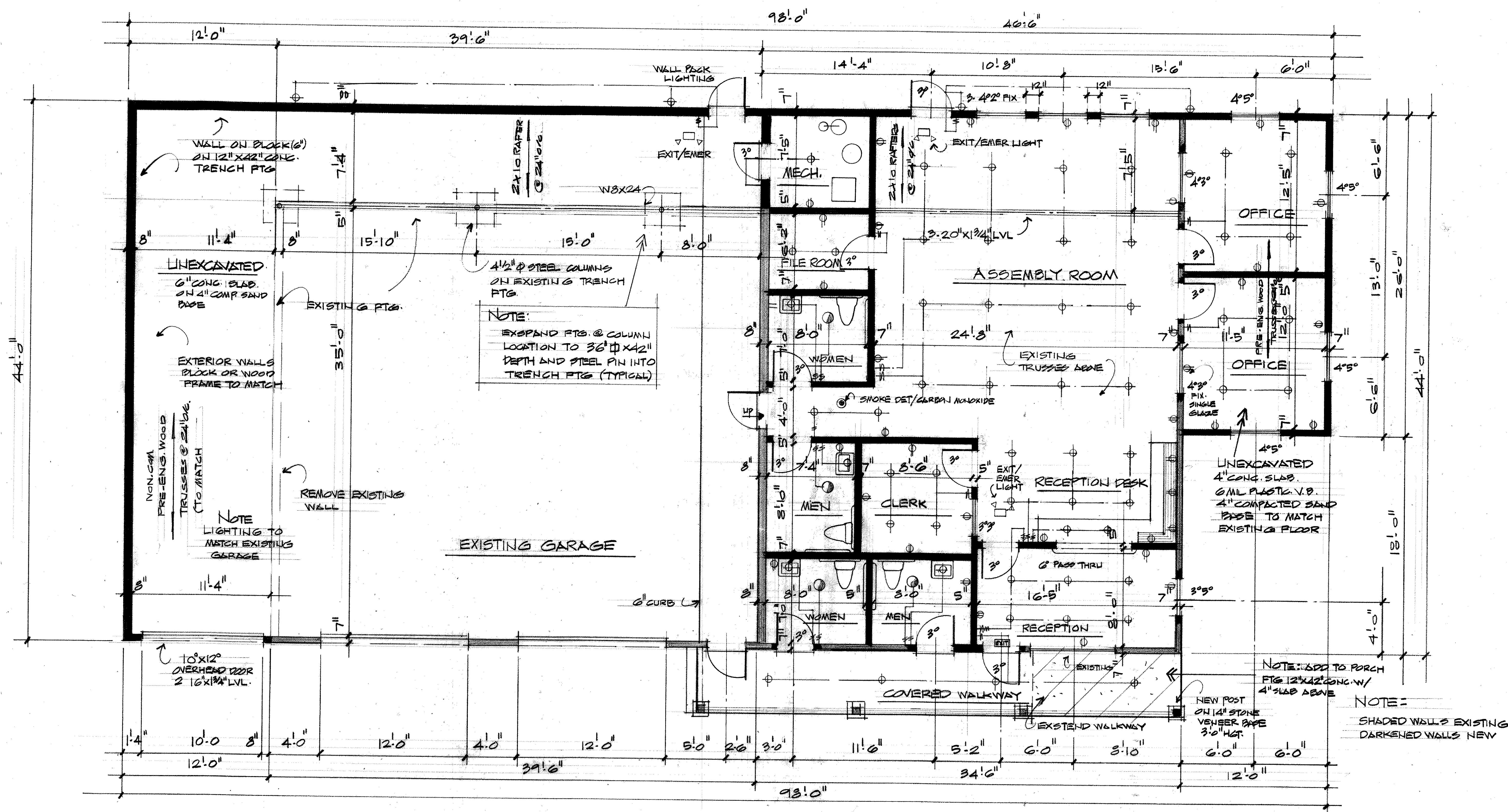
FLOOR PLAN 1/4" = 1'-0"
